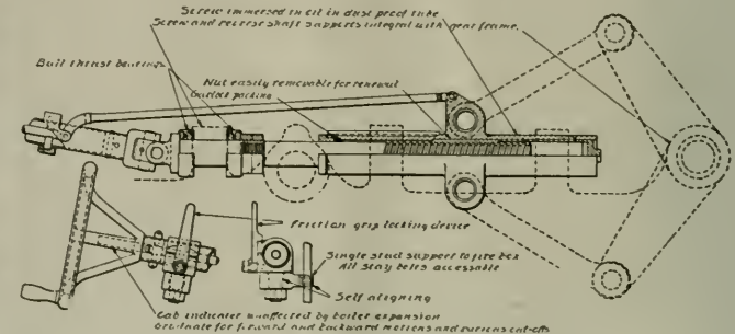
FIG. 4. SECTION VIEW OF THE REVERSE GEAR.
